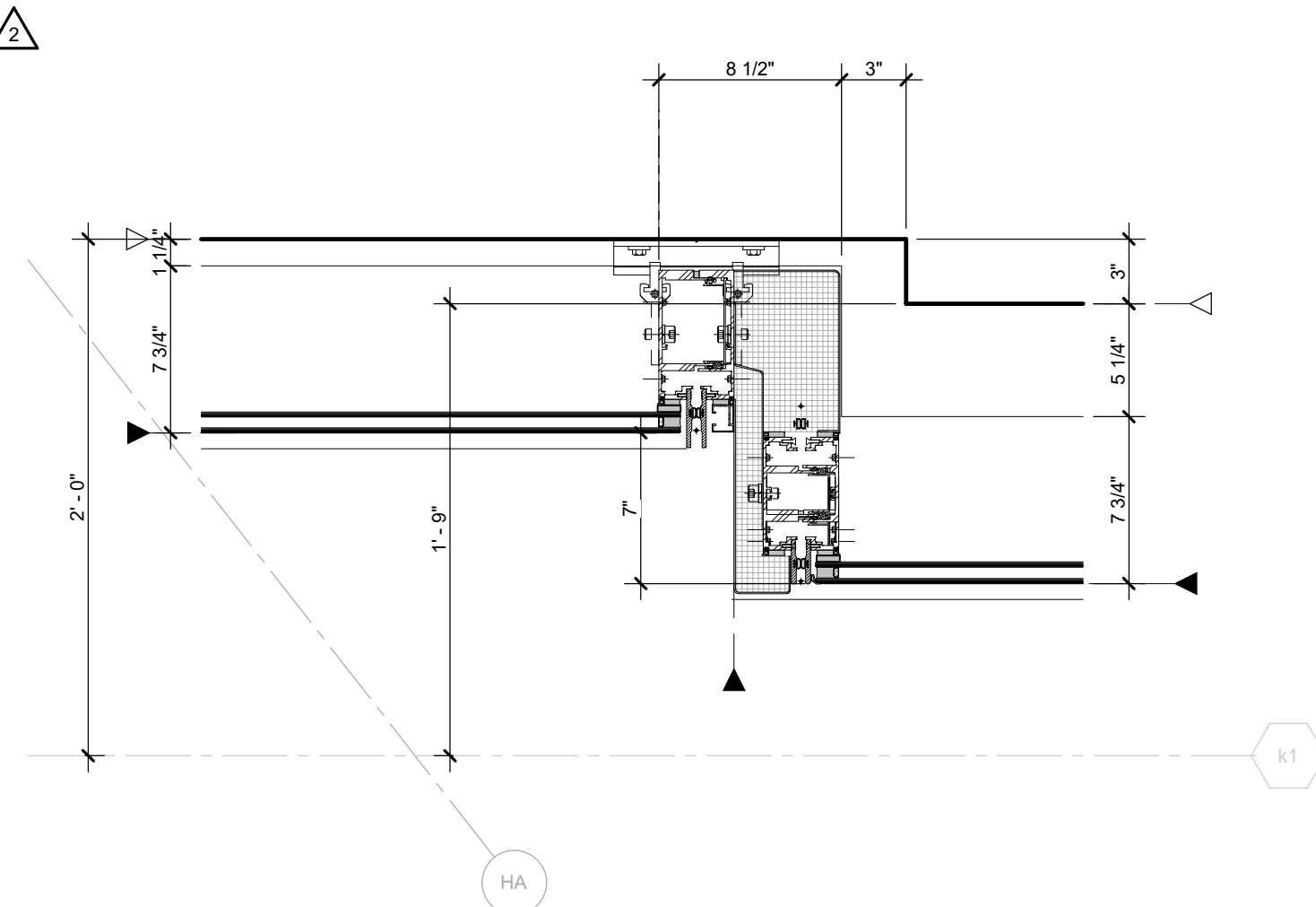
07 PLAN DETAIL - AT BRIDGE 1 1/2" = 1'-0"
