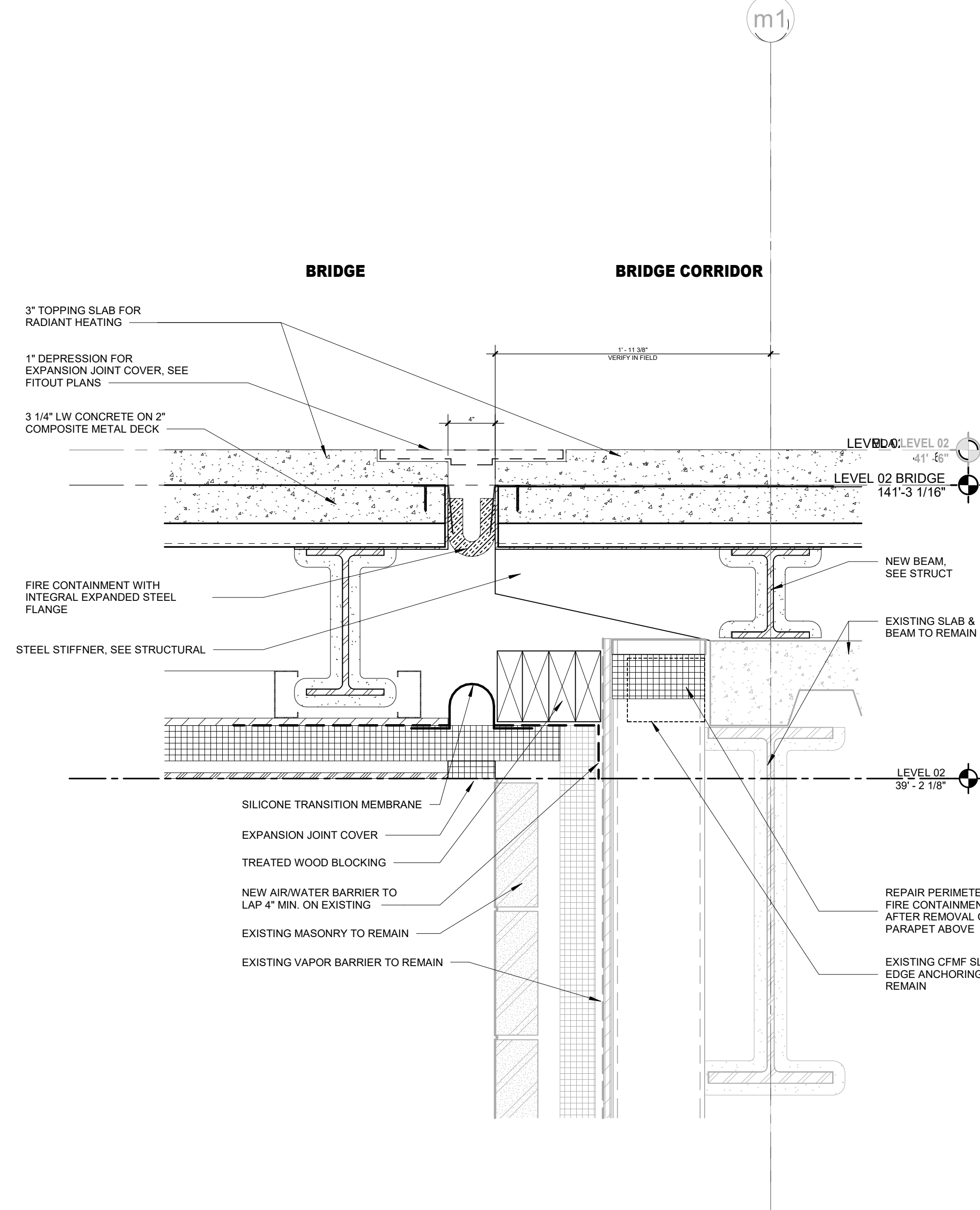
03 SECTION DTL - BRIDGE SLAB TO MD ANDERSON WEST FACADE 1 1/2" = 1'-0"
