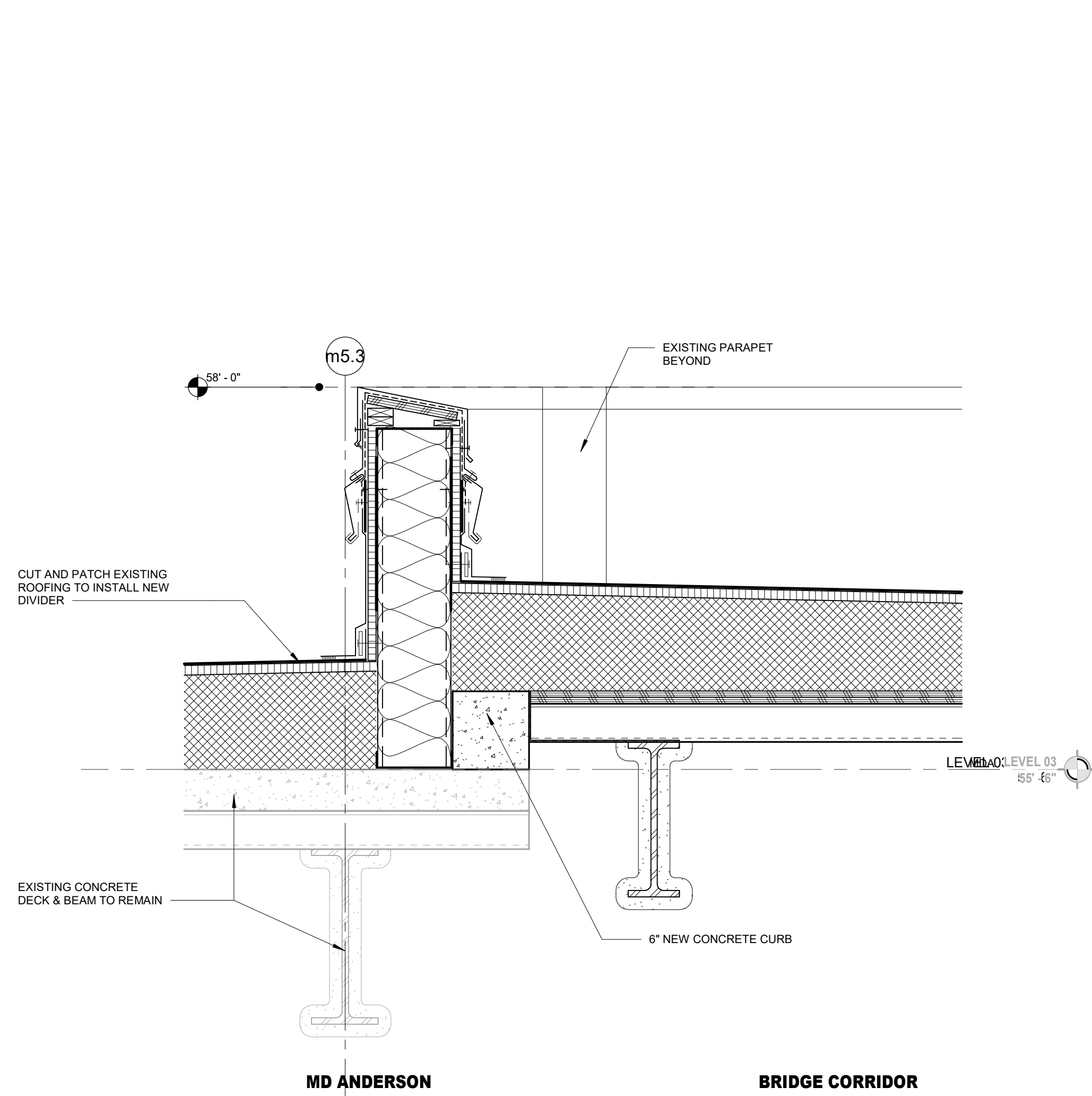
07 SECTION DTL - BRIDGE CORRIDOR ENTRY TO MD ANDERSON LVL 3 ROOF 1 1/2" = 1'-0"
