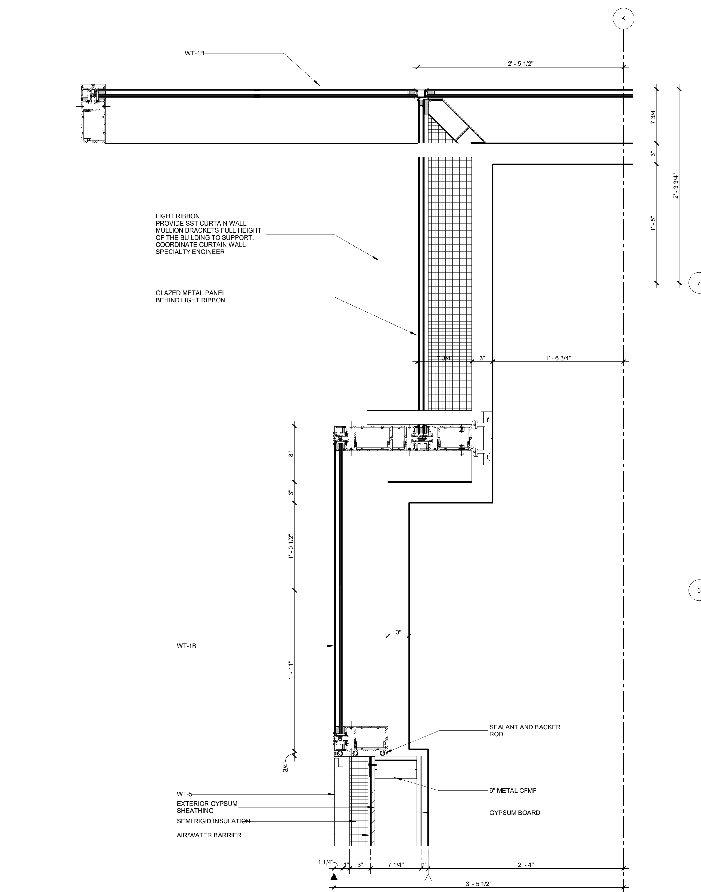
03 PLAN DETAIL - AT NW CORNER
