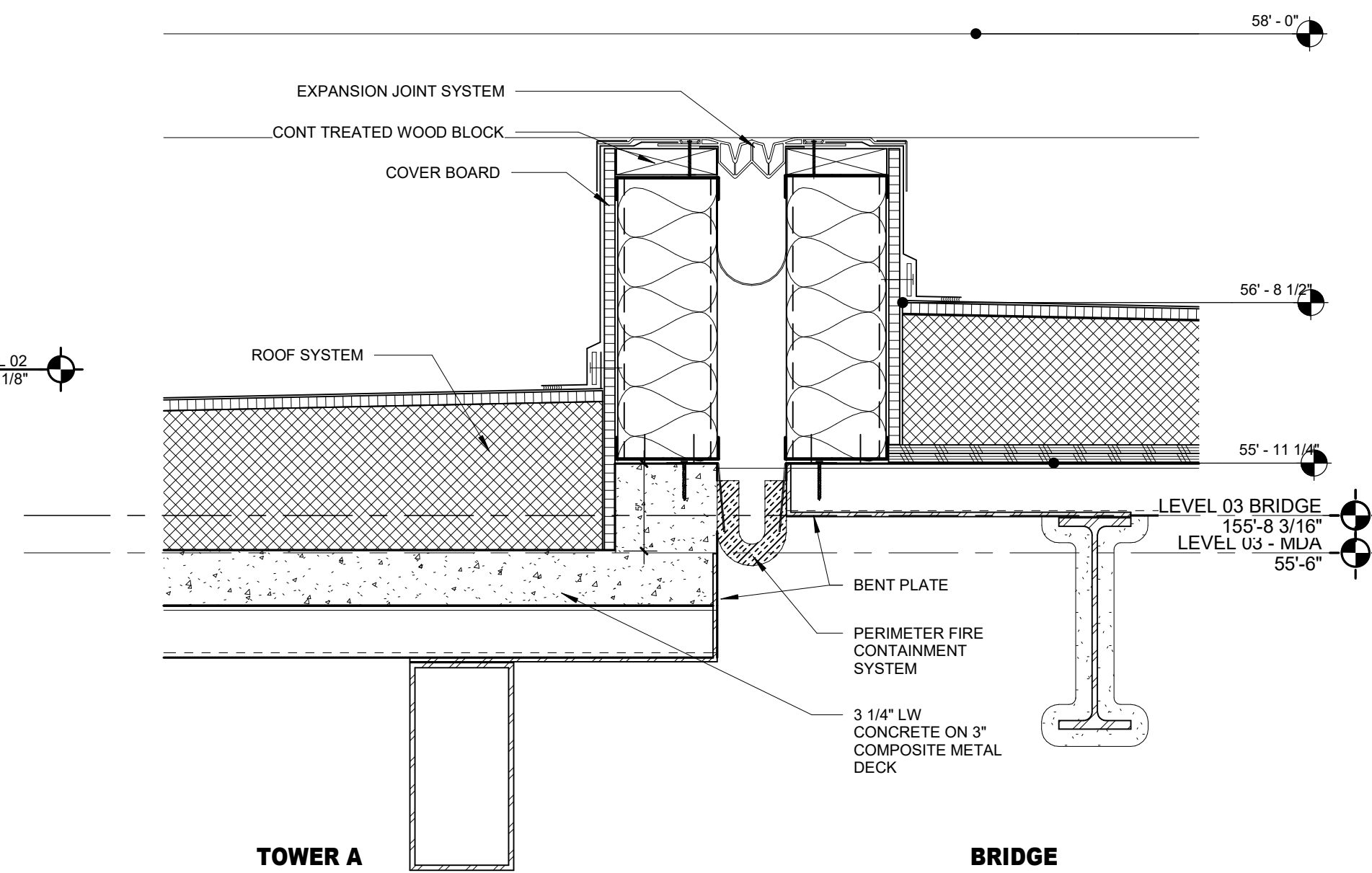
06 SECTION DTL - TOWER A / BRIDGE PARAPET EXPANSION JOINT 1 1/2" = 1'-0"
