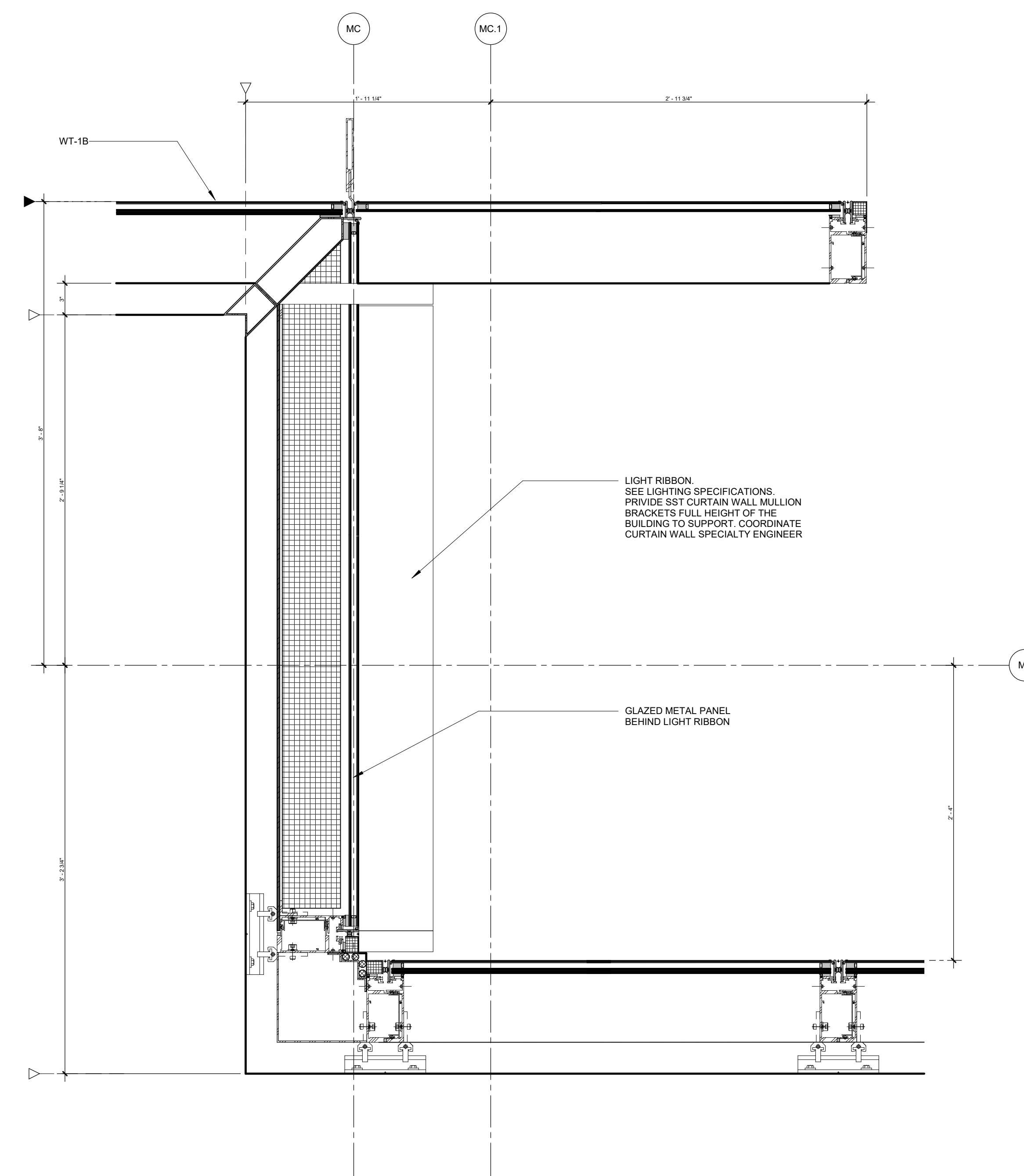
01 PLAN DETAIL - CW AT FLYBY LIGHTING RIBBON 1 1/2" = 1'-0"
