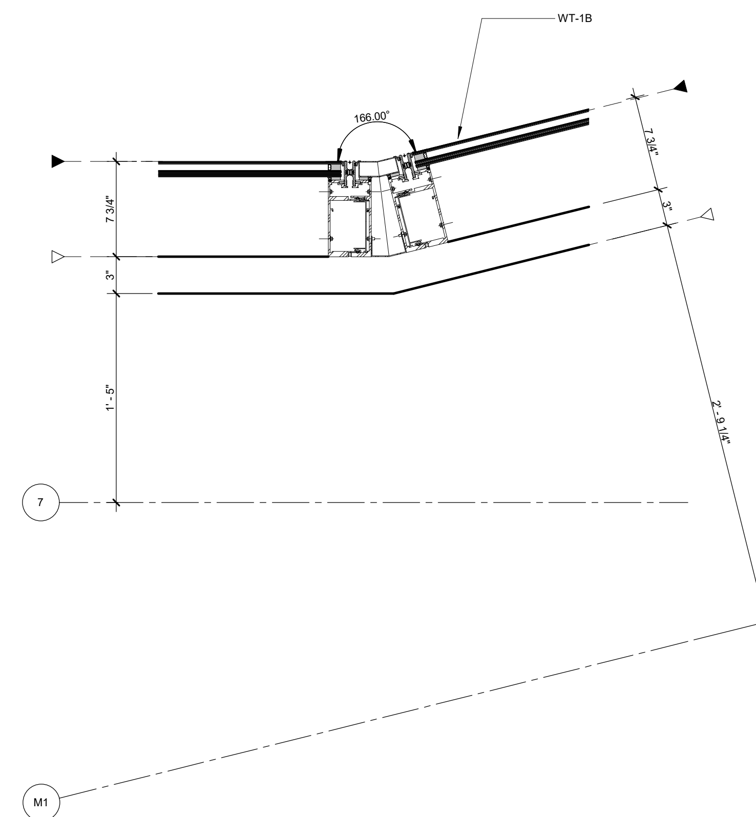
02 PLAN DETAIL - ANGLED CW AT NORTH FACADE
