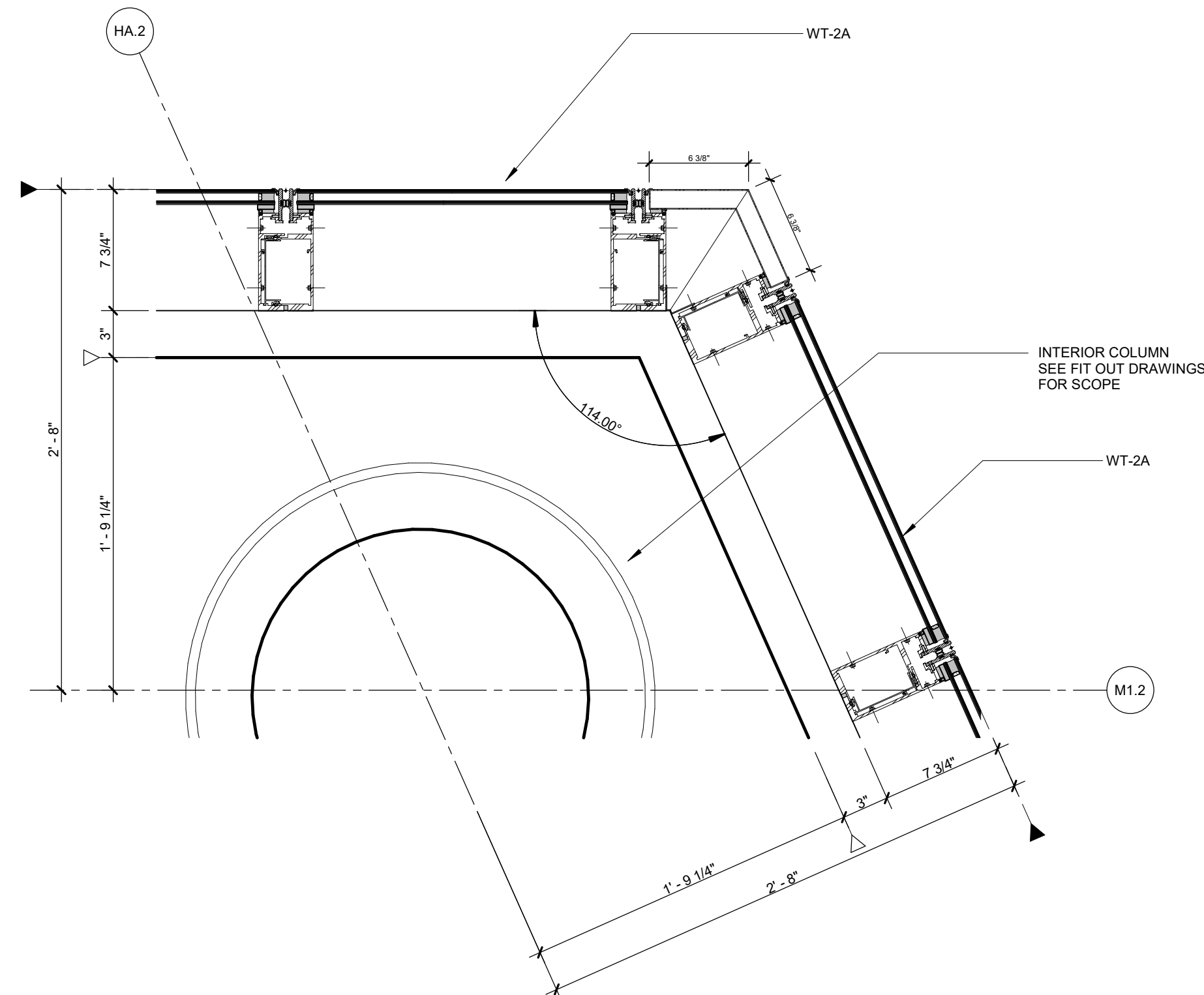
06 PLAN DETAIL - AT NE CORNER
