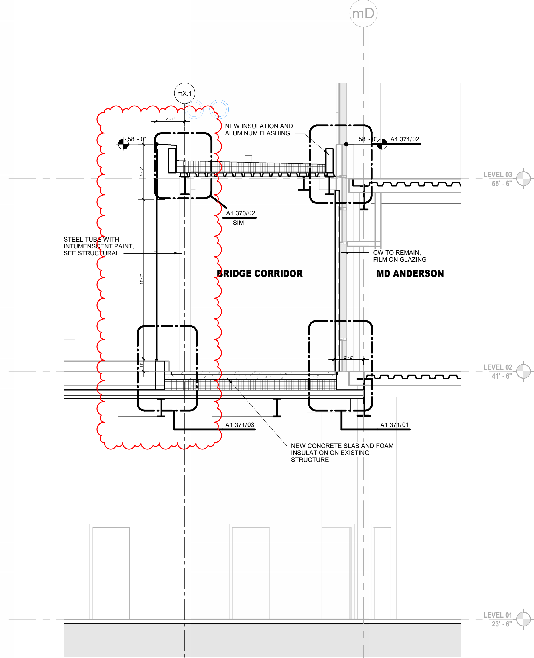
04 CROSS SECTION - THRU CORRIDOR AT MD ANDERSON 1/4" = 1'-0"
