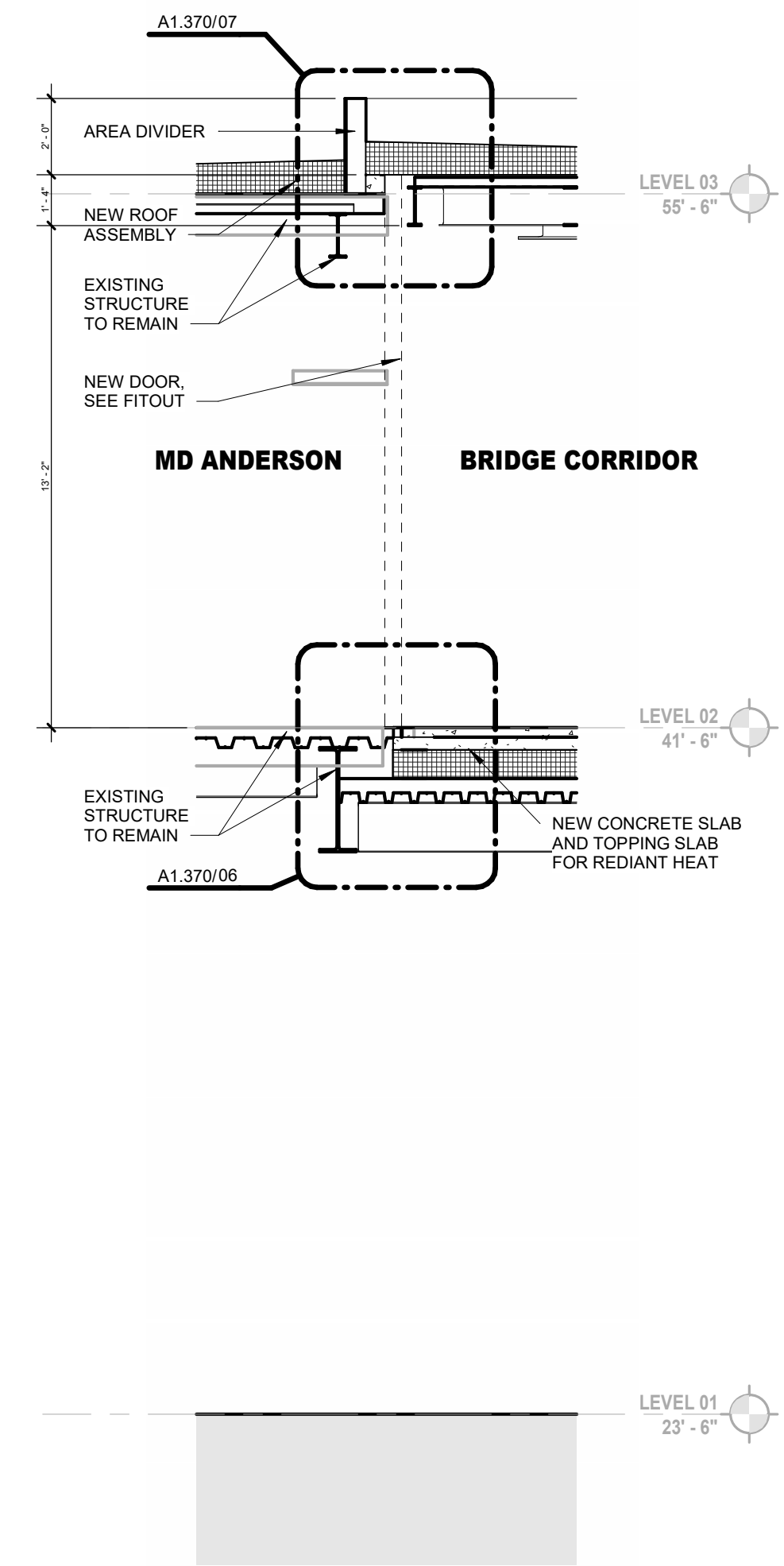
03 WALL SECTION - THRU THE BRIDGE CORRIDOR ENTRY AT MD ANDERSON 1/4" = 1'-0"
