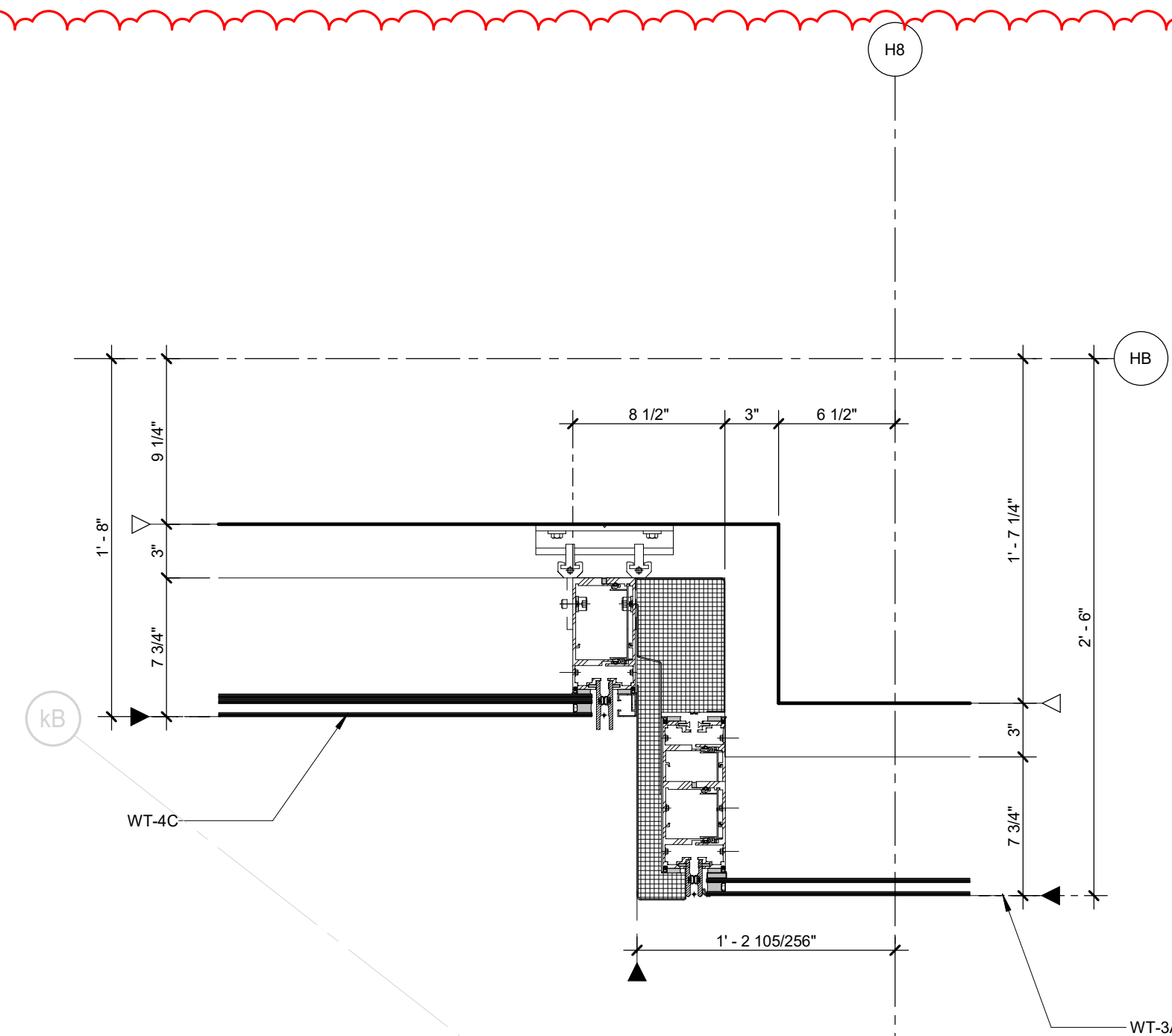
04 PLAN DETAIL - AT SE STAIR TOWER STACKED CW MULLION 1 1/2" = 1'-0"
