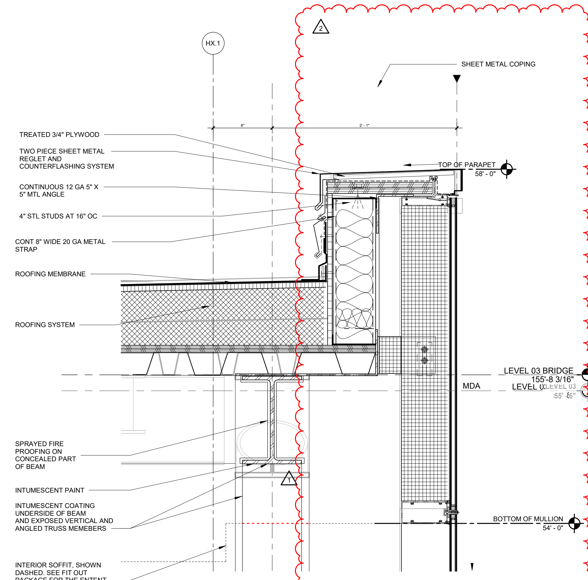
02 SECTION DTL - BRIDGE PARAPET 1 1/2" = 1'-0"
