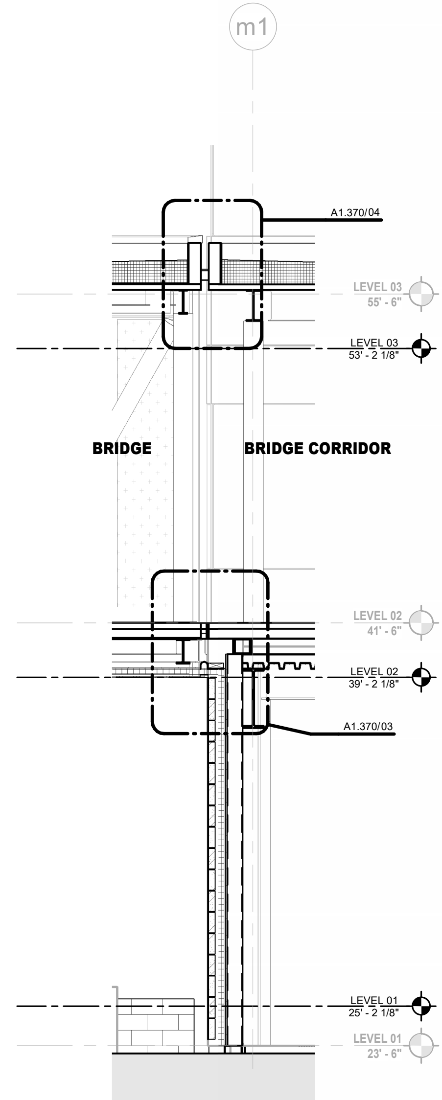
02 WALL SECTION - THRU MD ANDERSON FACADE 1/4" = 1'-0"
