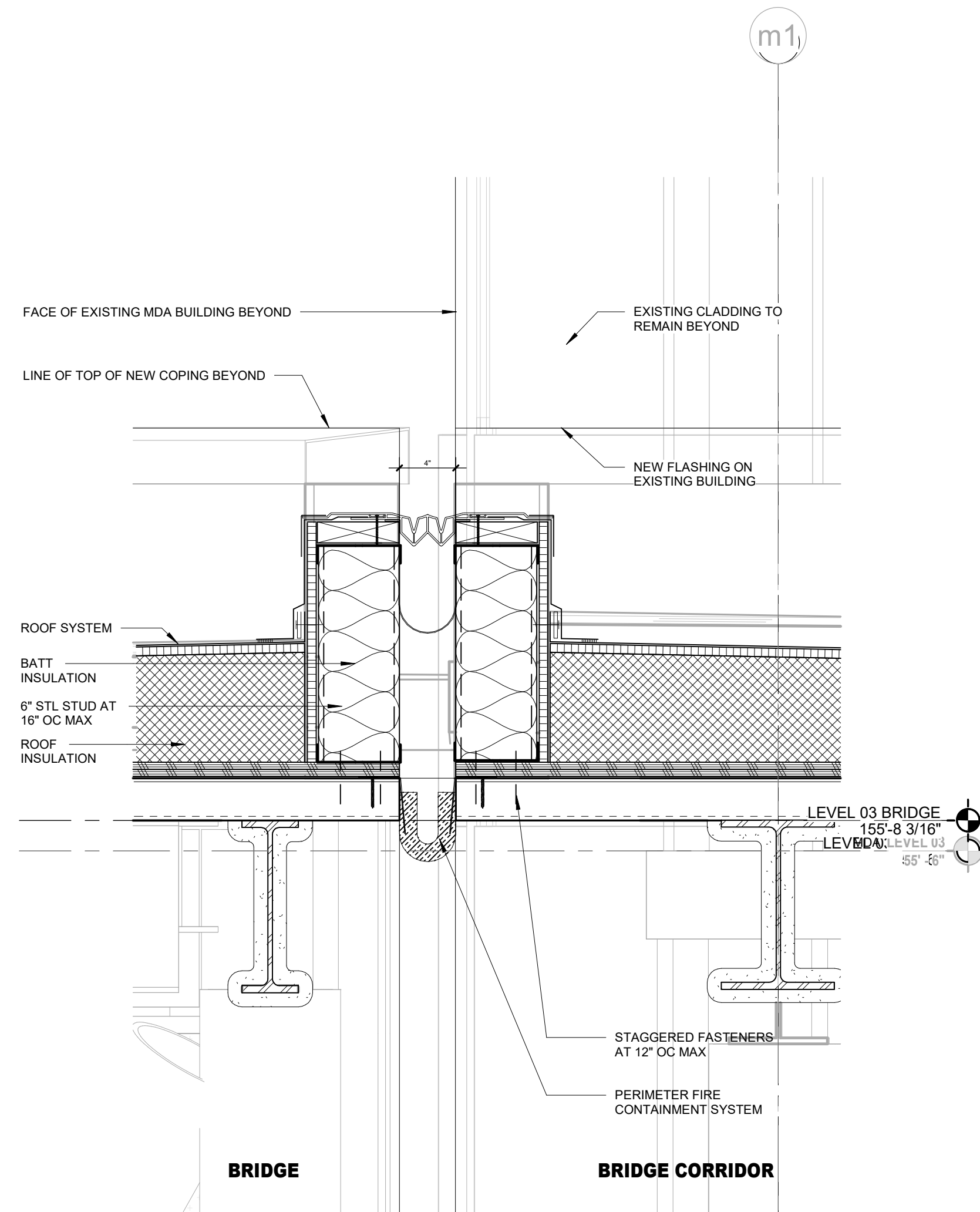
04 SECTION DTL - BRIDGE / BRIDGE CORRIDOR EXPANSION JOINT 1 1/2" = 1'-0"
