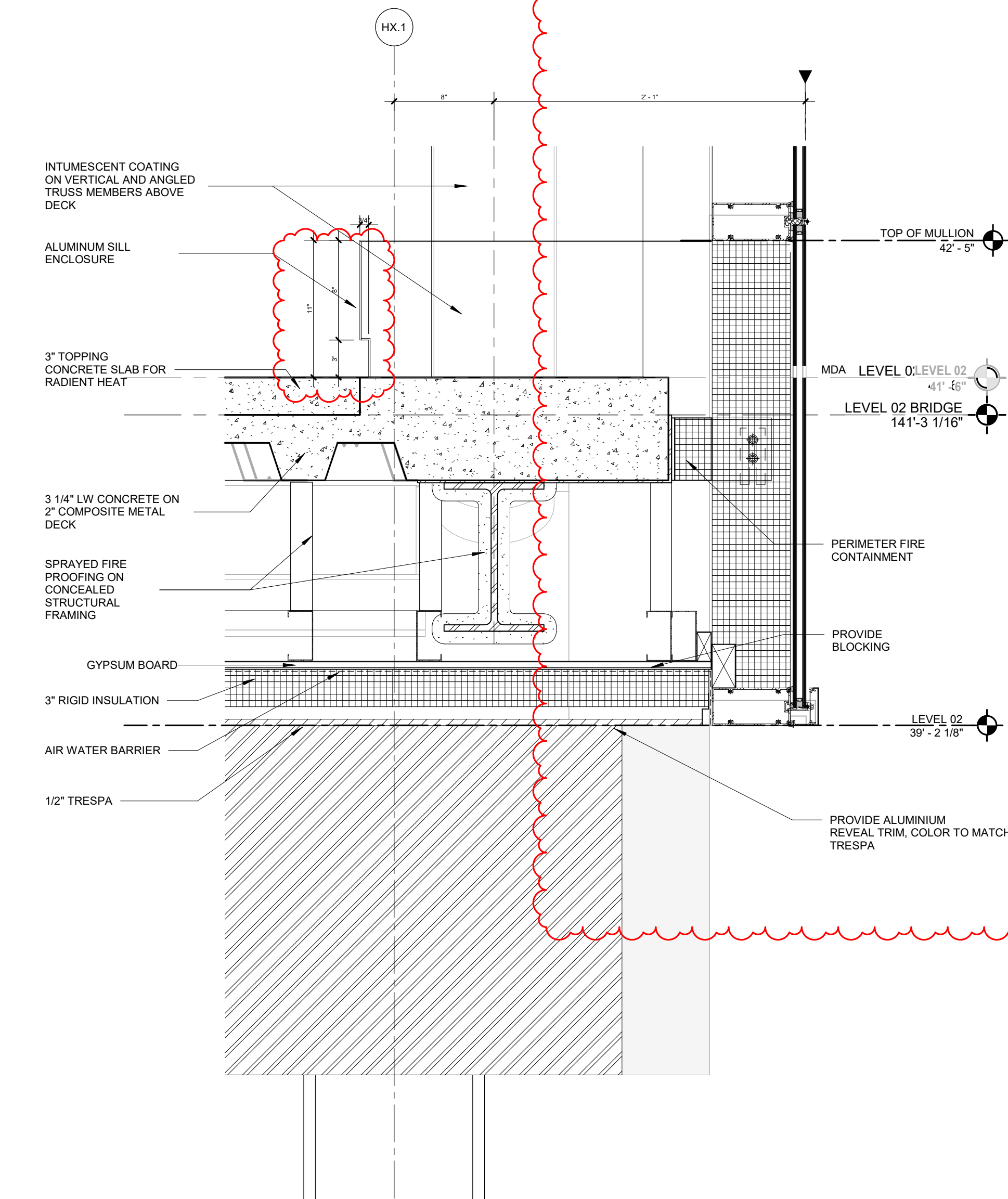
01 SECTION DTL - BRIDGE CW AT SLAB EDGE AND SOFFIT 1 1/2" = 1'-0"
