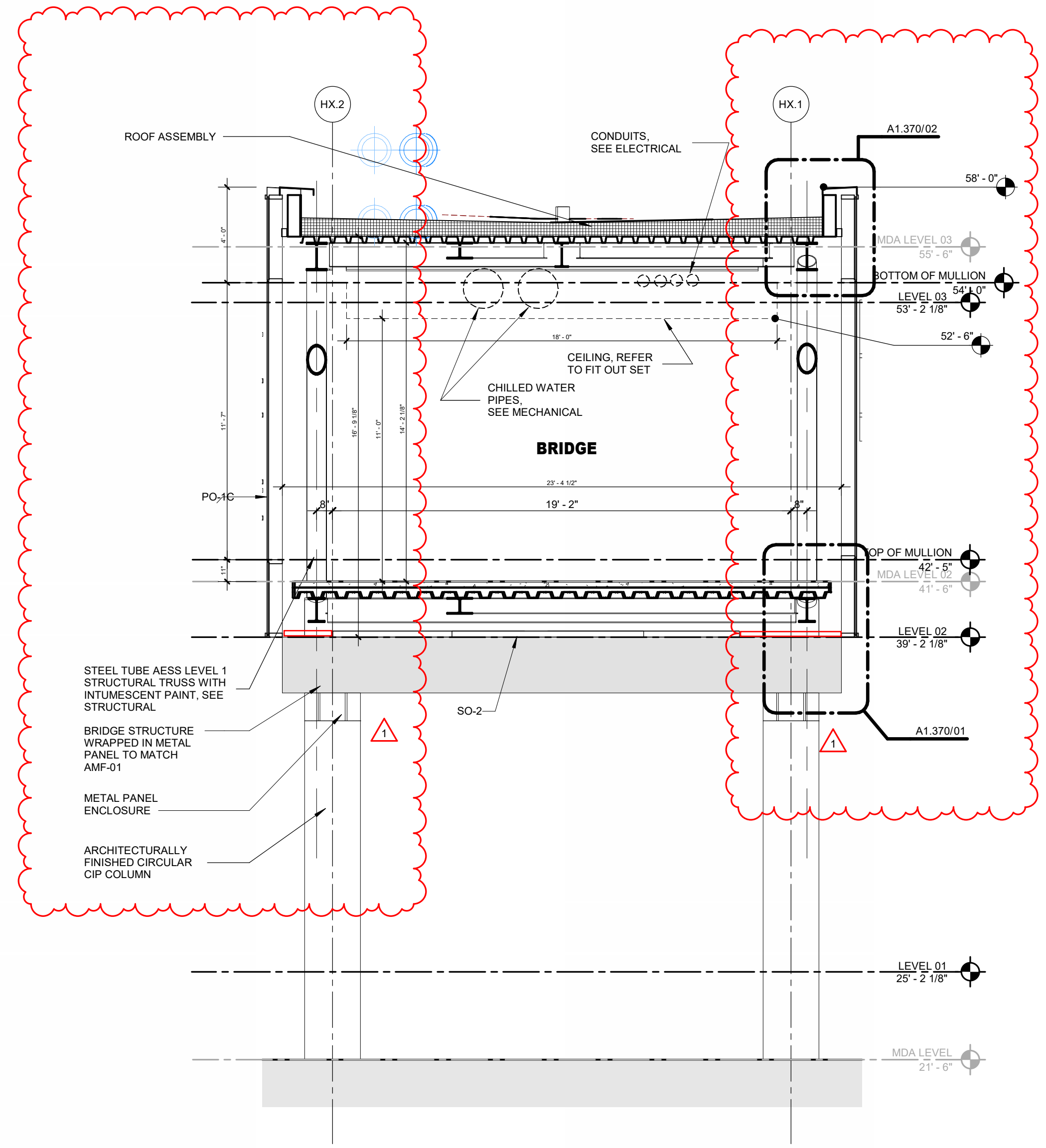
01 CROSS SECTION - THRU BR 1/4" = 1'-0"
