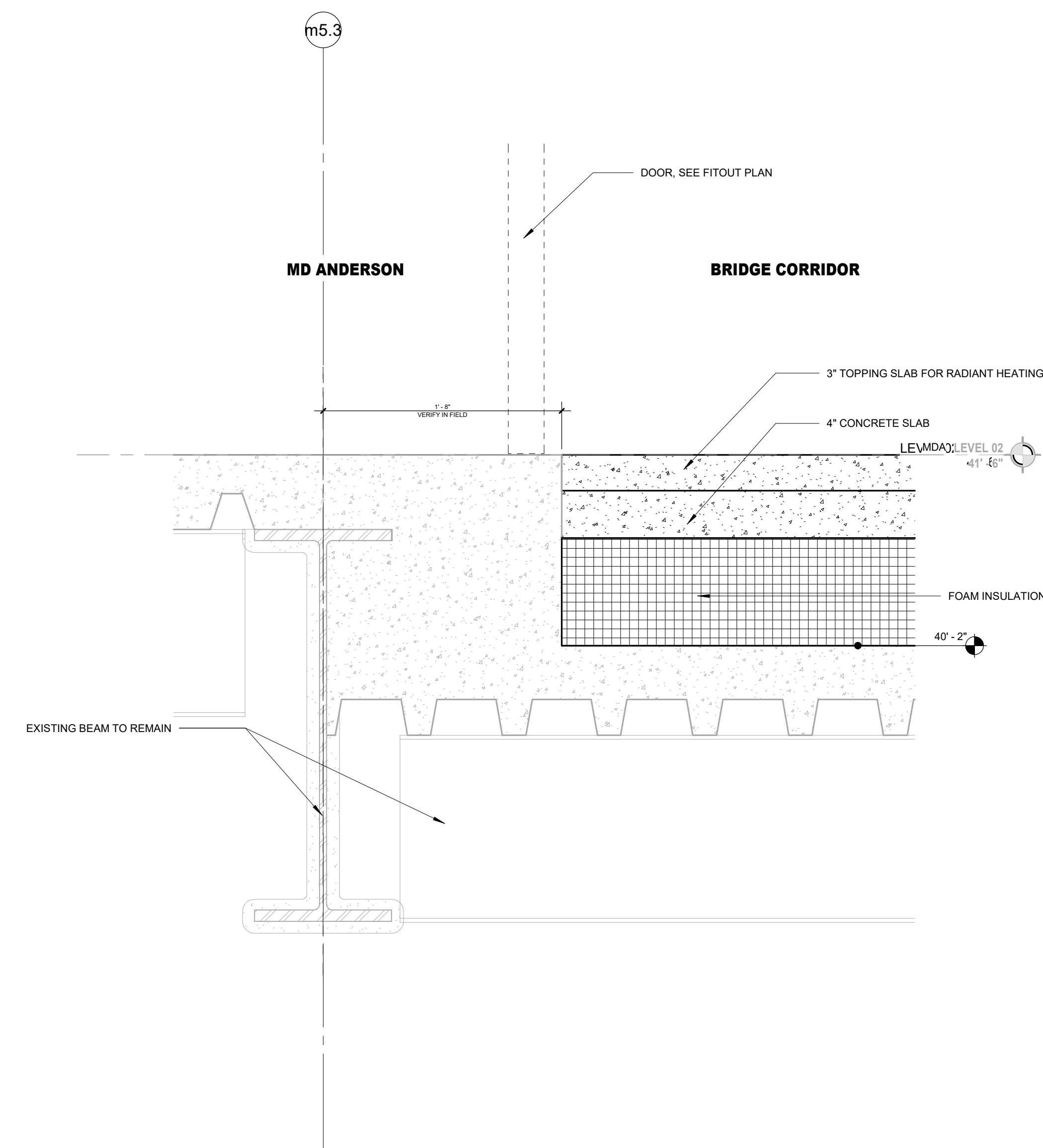
07 SECTION DTL - BRIDGE CORRIDOR ENTRY TO MD ANDERSON LVL 3 ROOF 1 1/2" = 1'-0"
